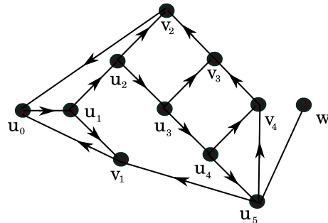
Figure 2: The kinked embedded lock K_x determined by the bit string x = 0111 .
